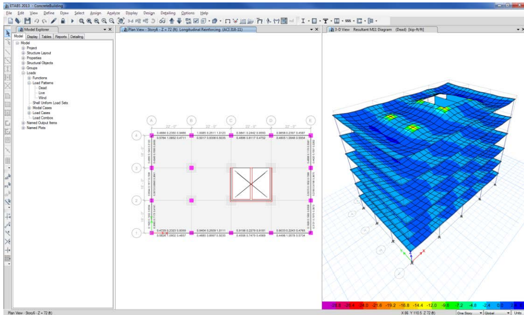
Figure 30 Longitudinal Reinforcing
