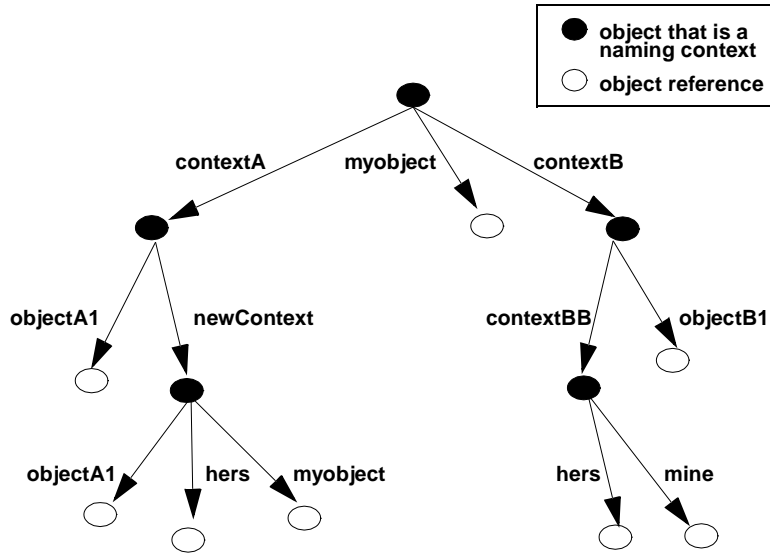
Example of a Naming Graph
